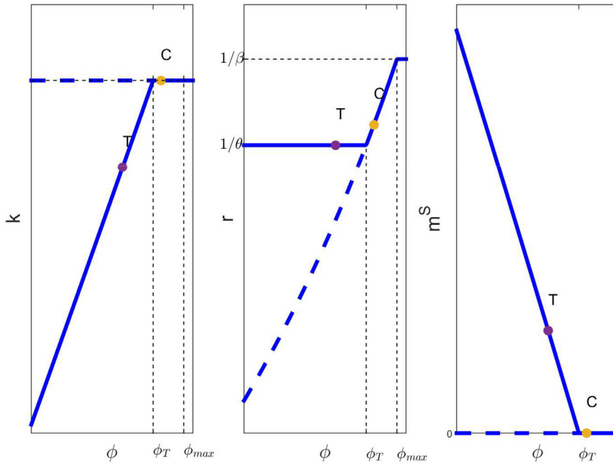
Fig. 2. Steady states - Comparative statics w.r.t. \phi , with \bar{l} = 0 .
