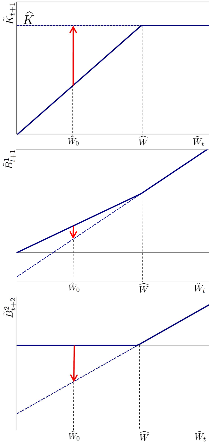
Figure 4: Convergence with g = g^*
